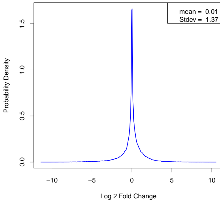
Probability Density of Fold Change. SEQC Sample A vs Sample B
