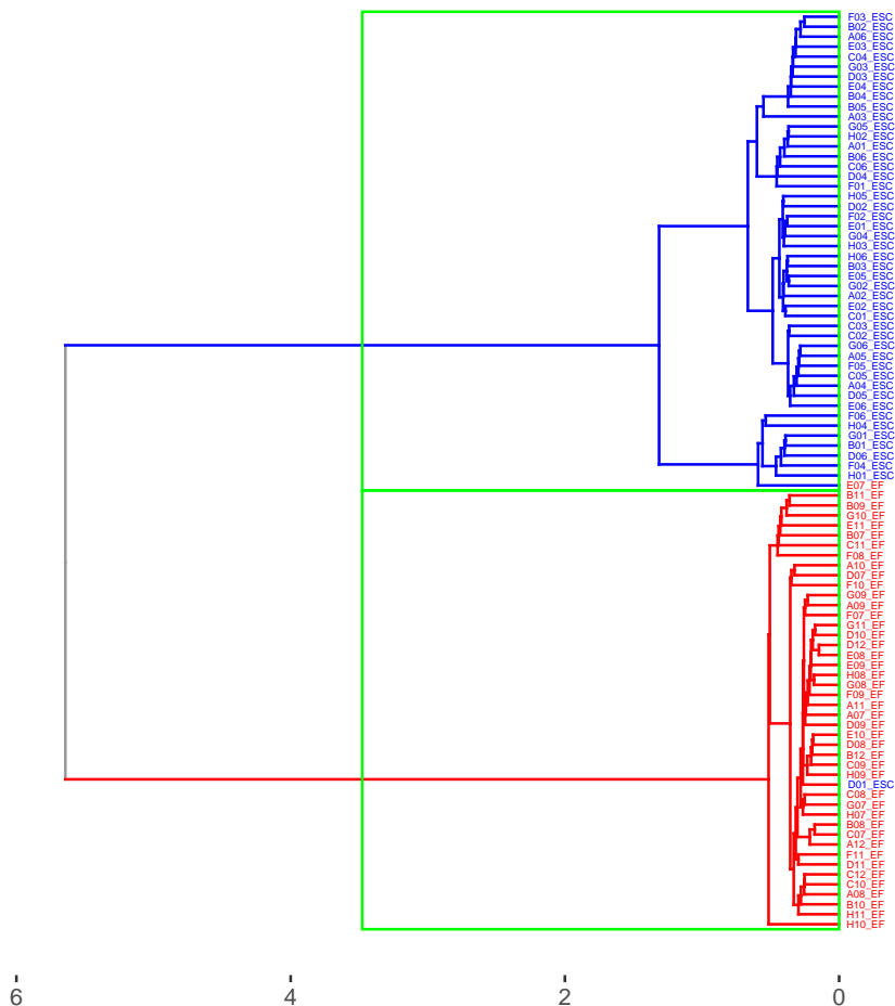
Hierarchical clustering
