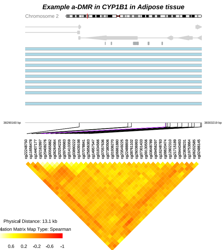
Figure 4: Plot with comet function without pvalue plot.
