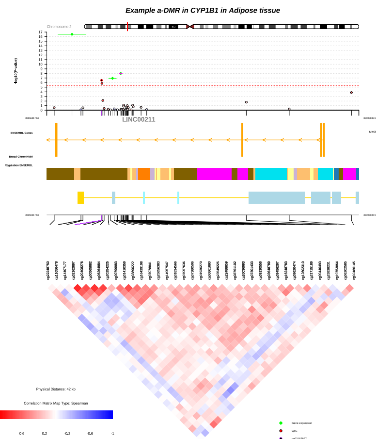
Figure 1: Plot with comet.web function.
