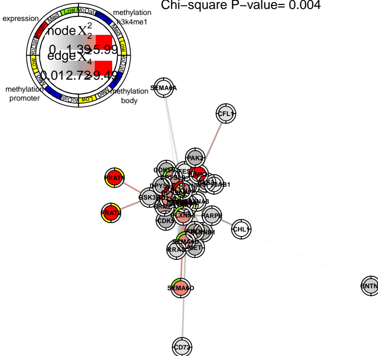
Network built around DPYSL4:NRP1:SEMA3A Chi-square P-value= 0.004
