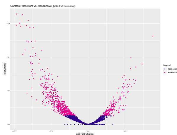
Figure 15: Volcano plot of Resistant-Responsive contrast, using a multi-factor design "Tissue + Condition" Sites identified as significantly differentially bound shown in magenta. Generated by: dba.plotVolcano(tamoxifen)
