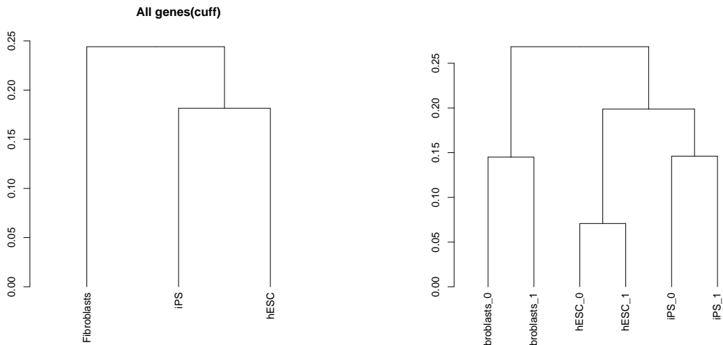
(a) Dendrogram of JS distances between conditions.
