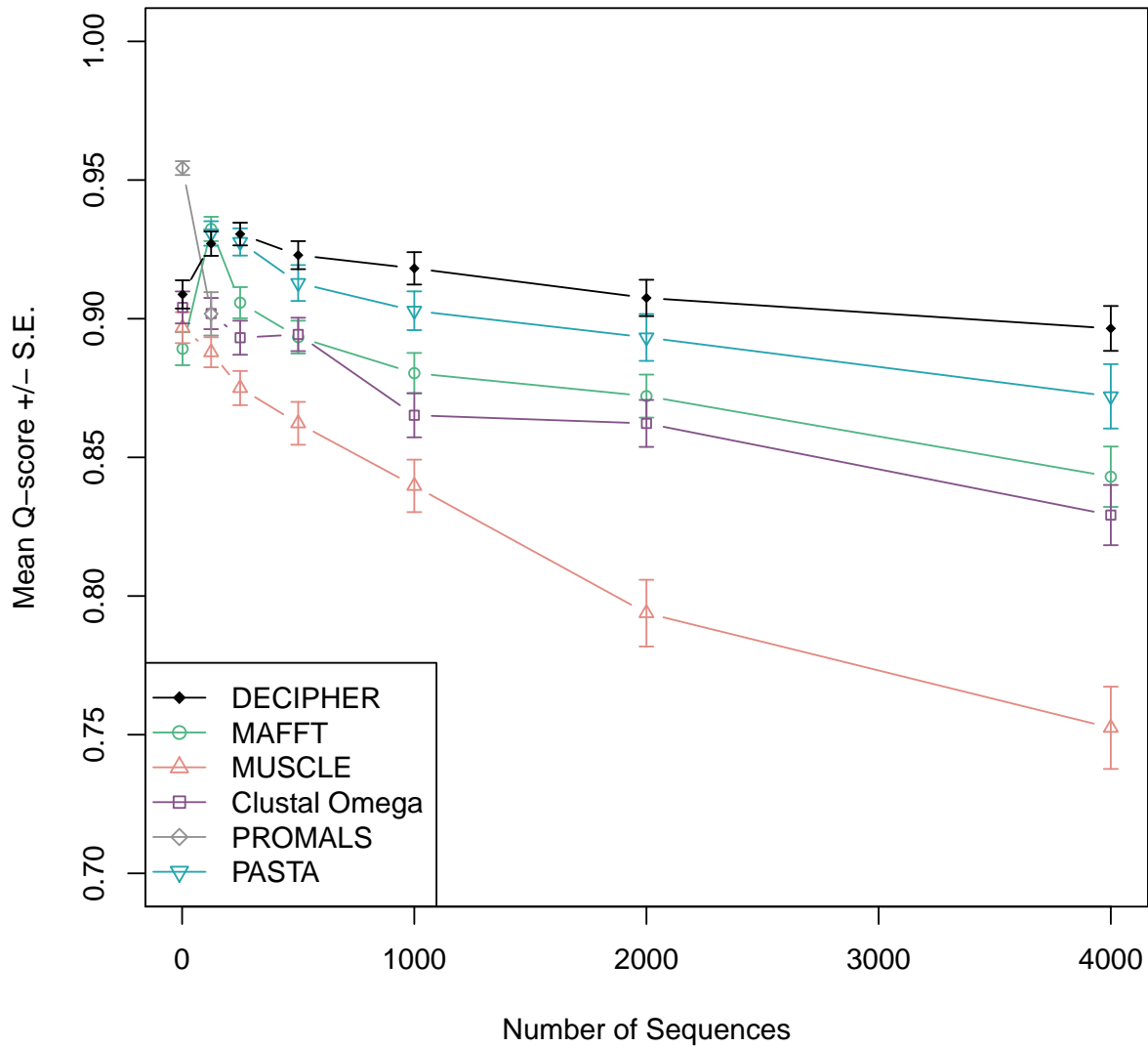
Figure 5: DECIPHER offers improved accuracy over other alignment programs ( [3, 5–7, 9, 13] ) on large sets of input sequences. Average accuracy on the Homstrad-mod benchmark [13] is shown for an increasing number of input sequences, ranging from 2 to 4,000. All programs display a peak in accuracy at fewer than 500 sequences, but DECIPHER exhibits the least drop-off in accuracy as additional input sequences are added.
