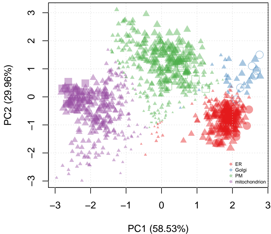
Figure 12: Representation of the svm prediction on the 888 data set. The svm scores have been used to set the point size ( cex argument; the scores have been transformed to emphasise the extremes). Different symbols ( fpch ) are used to differentiate markers and new assignments.
